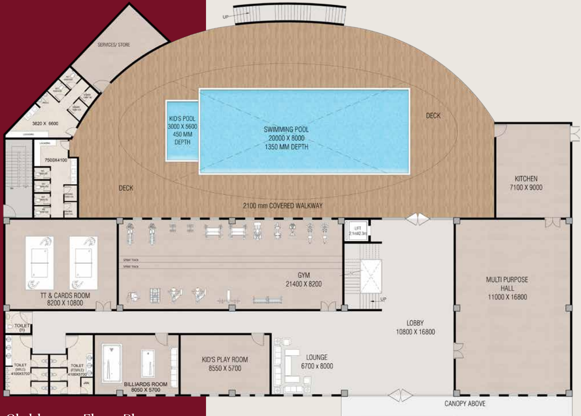
Clubhouse Floor Plan
